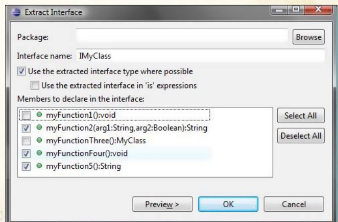
Figure 4. Extract interface
