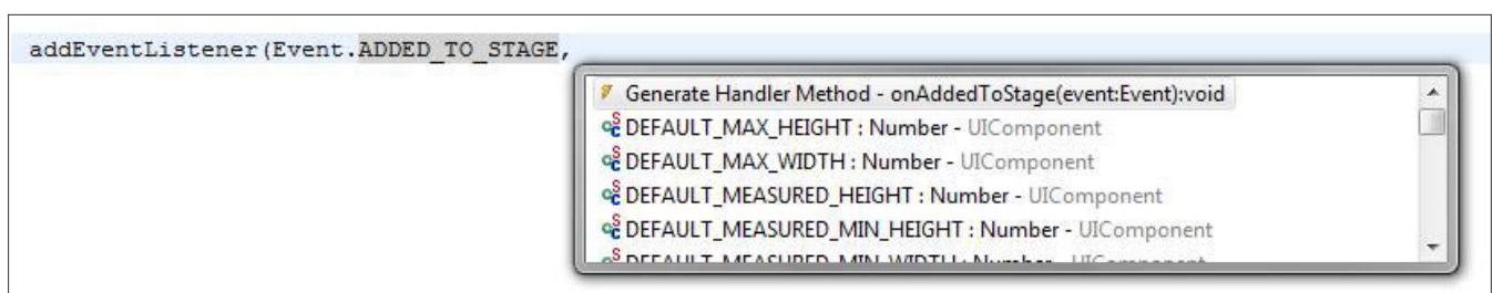
Figure 1. addEventListener
