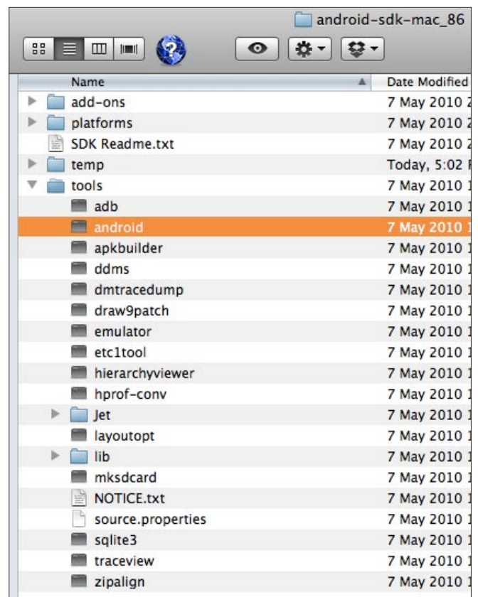
Figure 1. Android SDK
