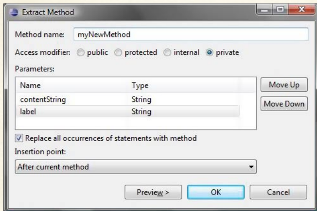
Figure 5. Extract method
